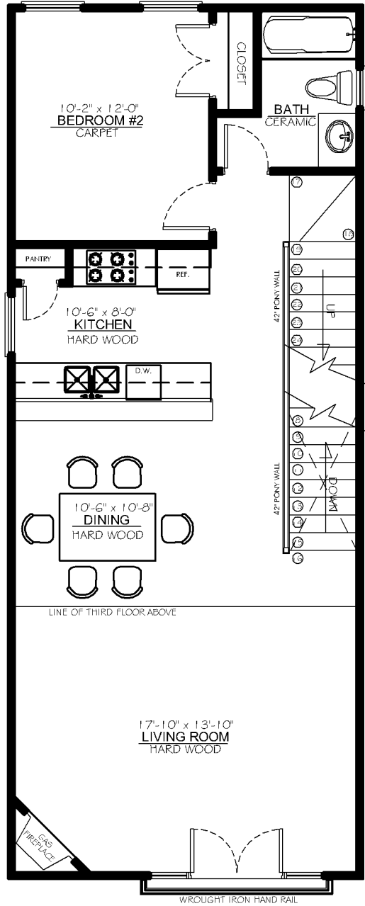
SECOND FLOOR 840 S.F.
